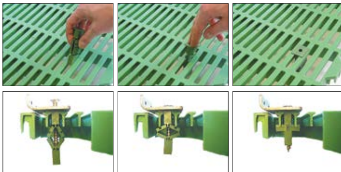
Mounting of rhomb anchor - article nr. 18958
