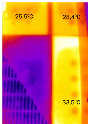
Thermographical heat distribution for plastic heating plate
